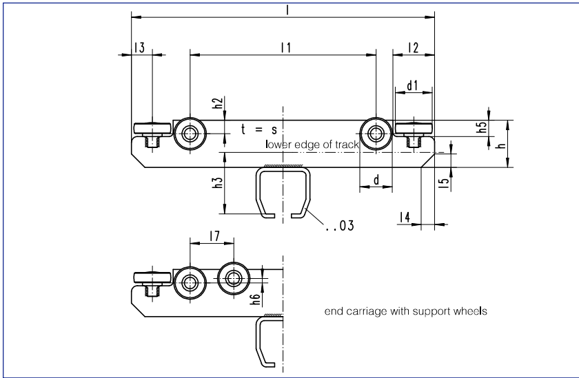
End carriage 1354-1754
