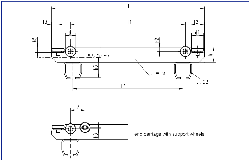
End carriage 1354/3-1754/3
